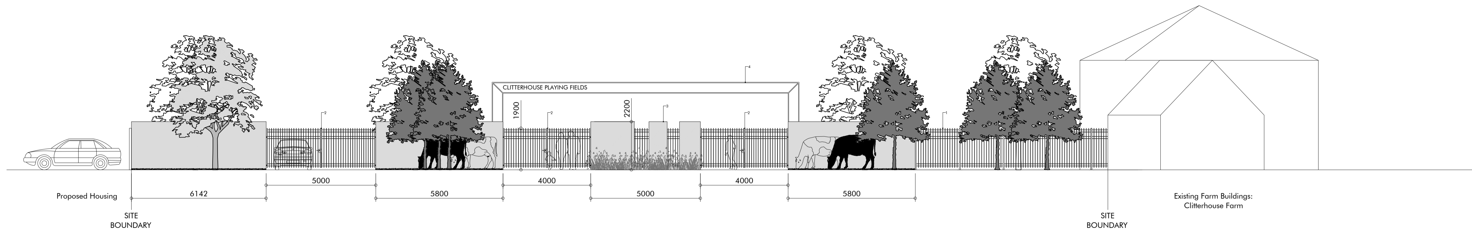
Elevation A - AA: Main Entrance 1:100 @ A1
