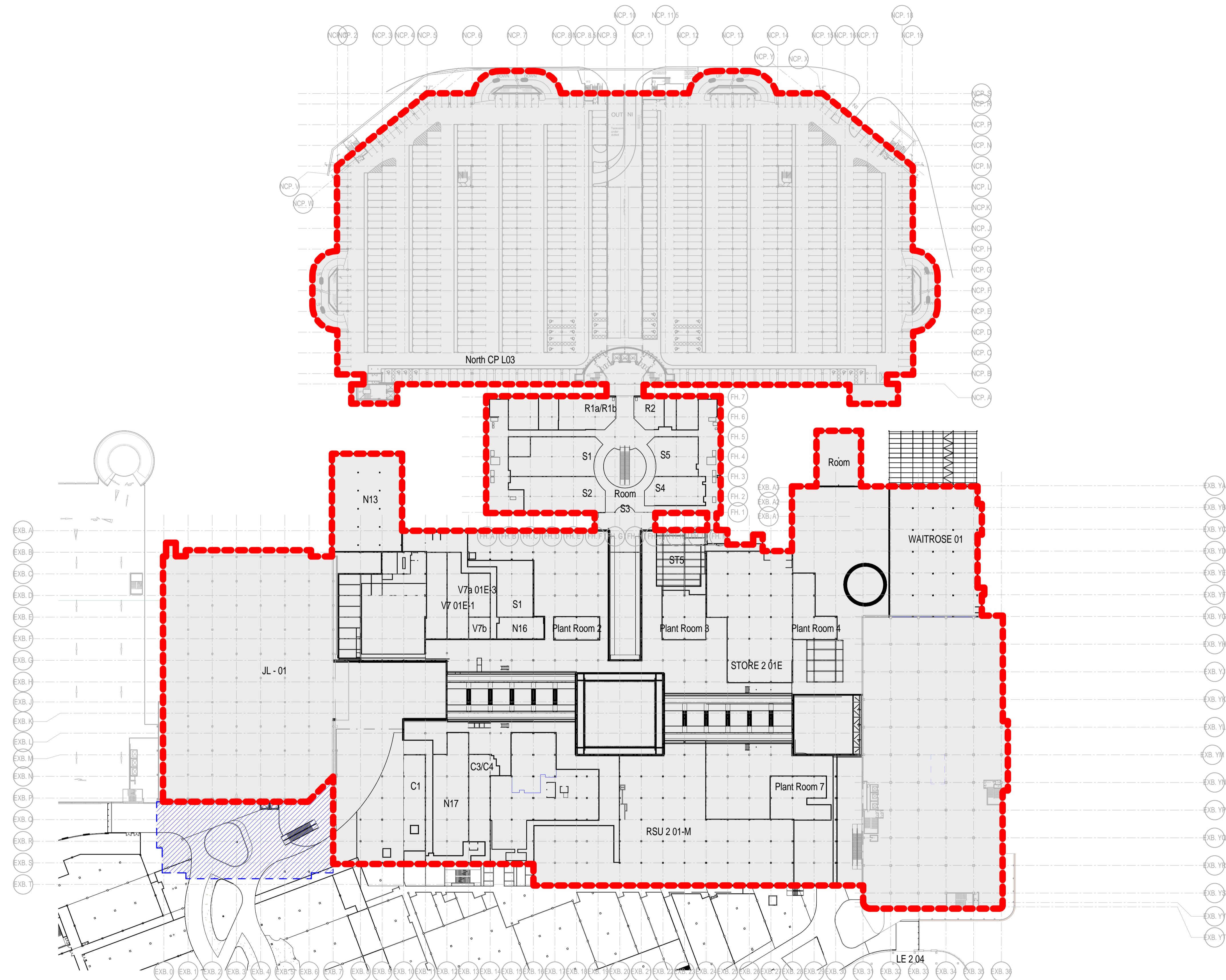
1 LEVEL 01 PLAN 1: 750
