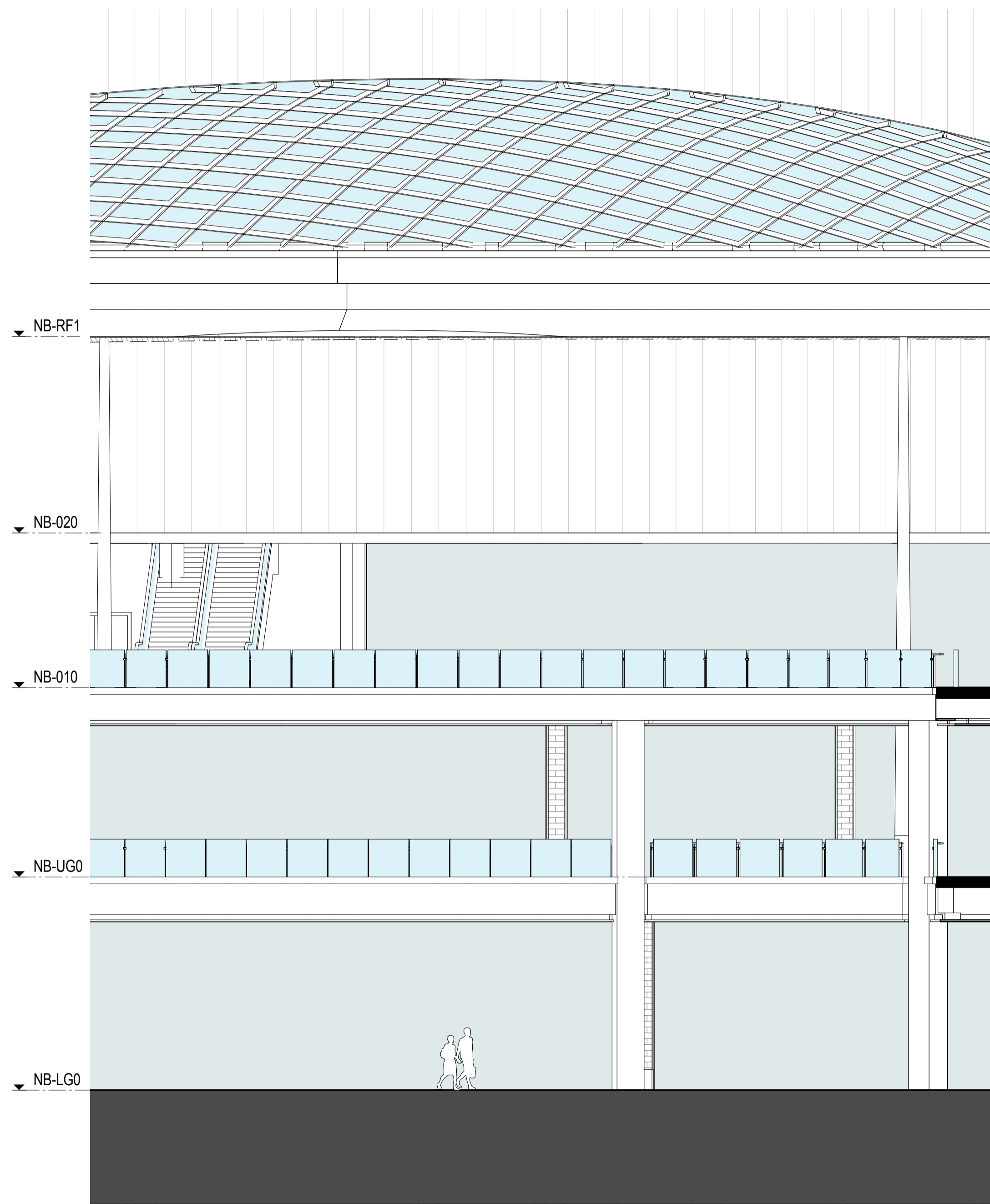
2 MAIN SQUARE ELEVATION ENLARGED 1:100
