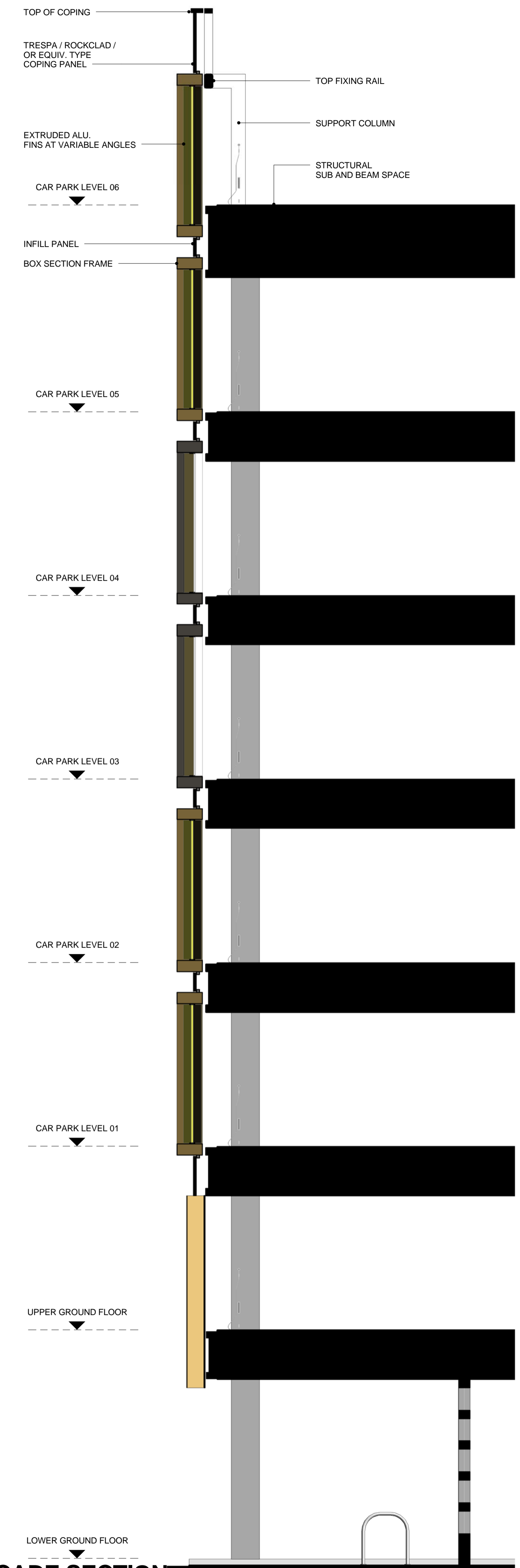
2 WEST FACADE SECTION 1 : 50
