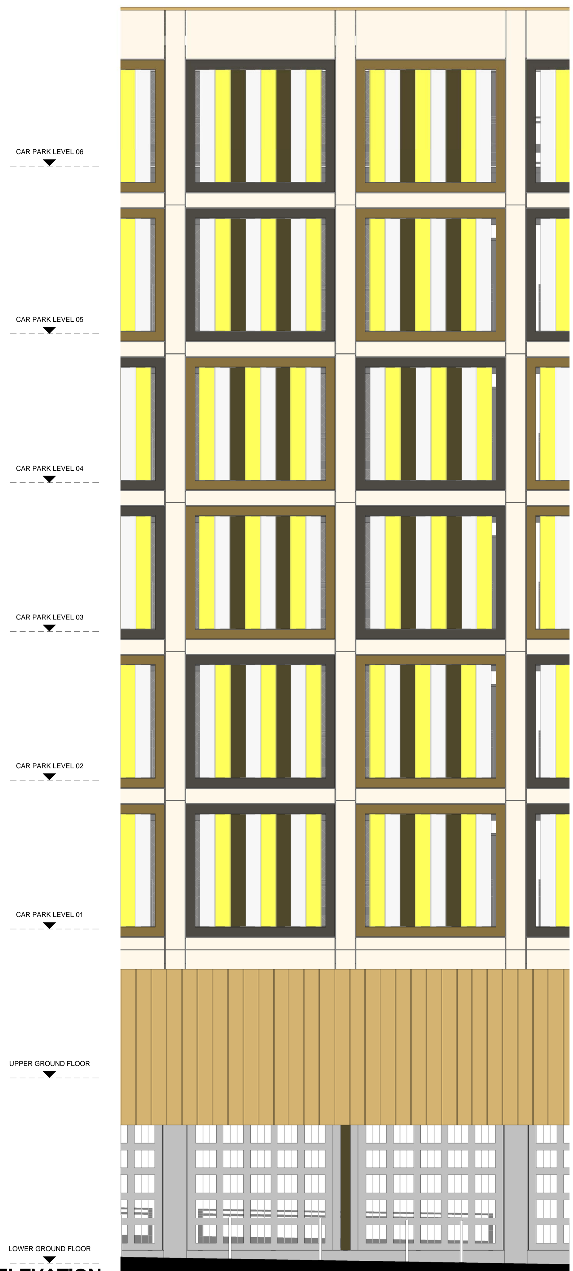
1 WEST FACADE BAY ELEVATION 1 : 50
