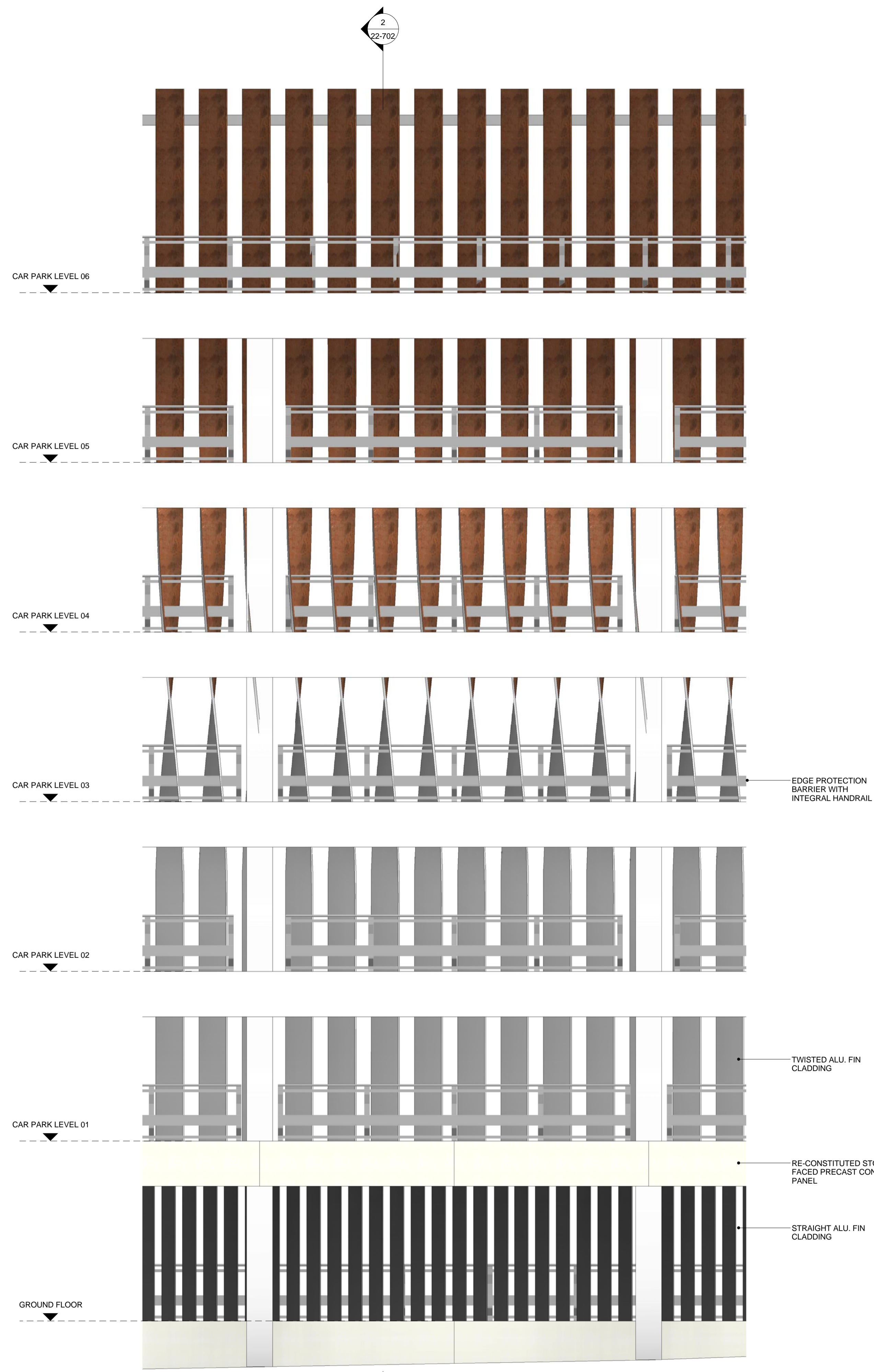
1 ELEVATION - FACADE STUDY 1 : 50
