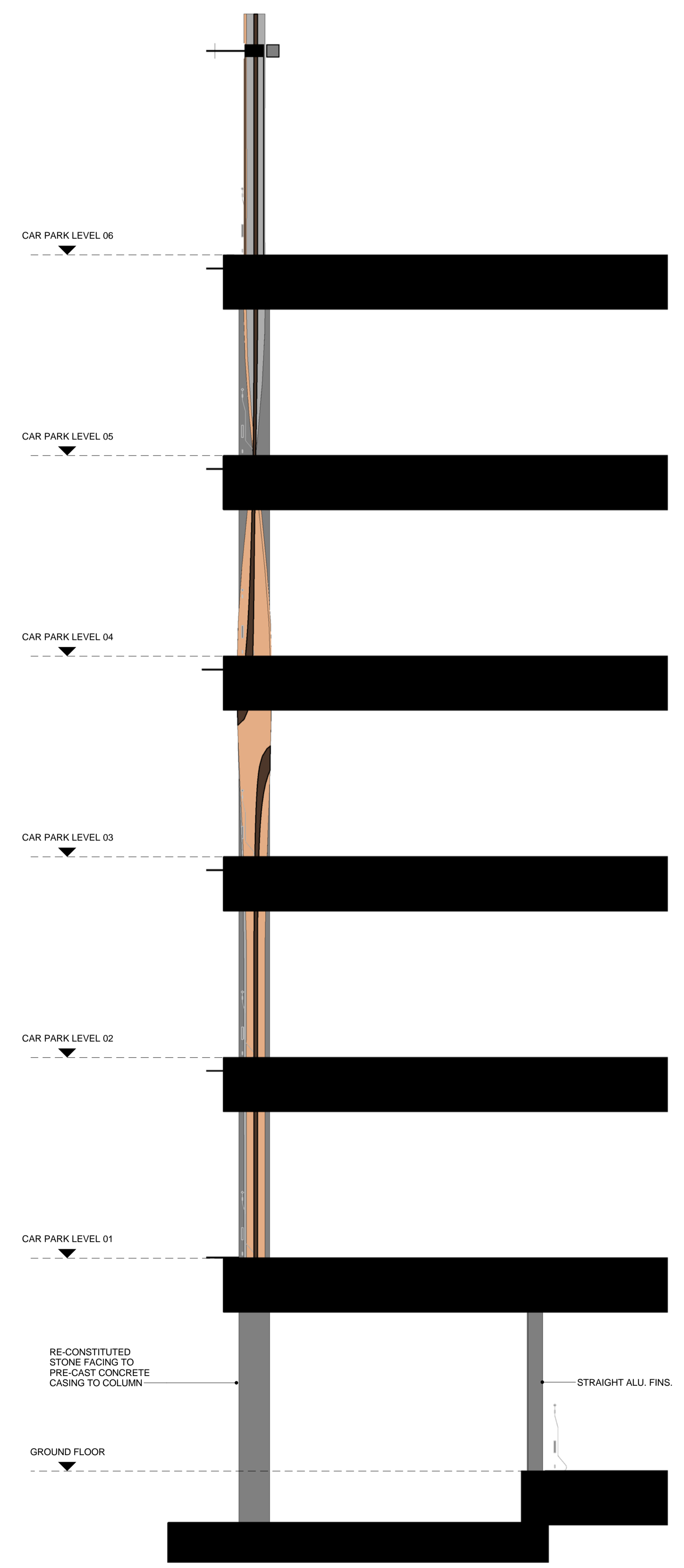
2 SECTION - FACADE SECTION 1 : 50
