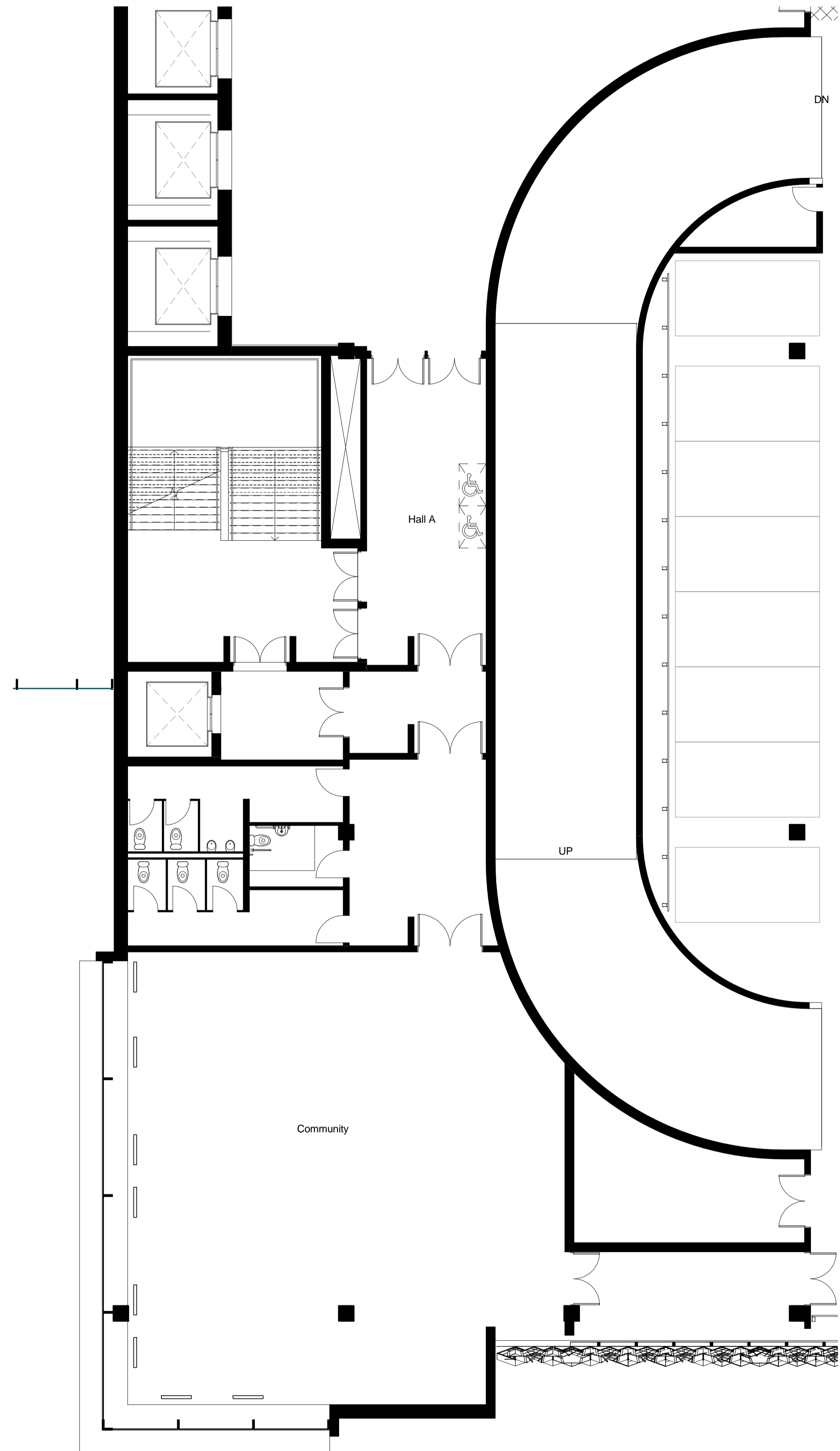
1 Community Study Plans - Level 2 (CP2) 1 : 100
