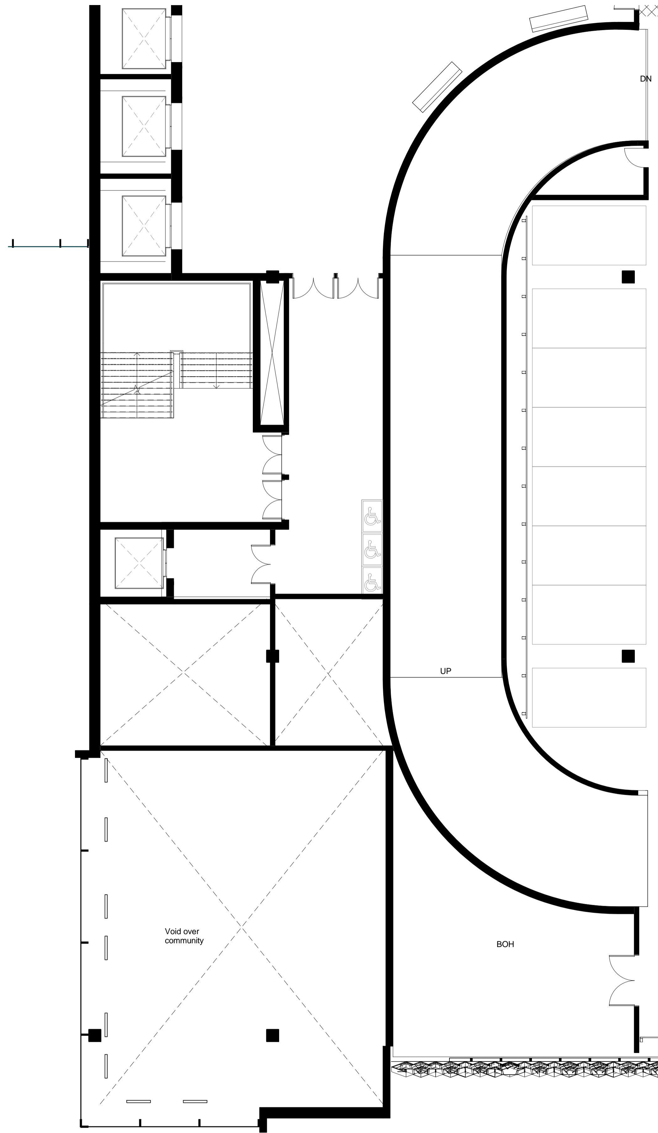
2 Community Study Plans - Level 3 (CP3) 1 : 100
