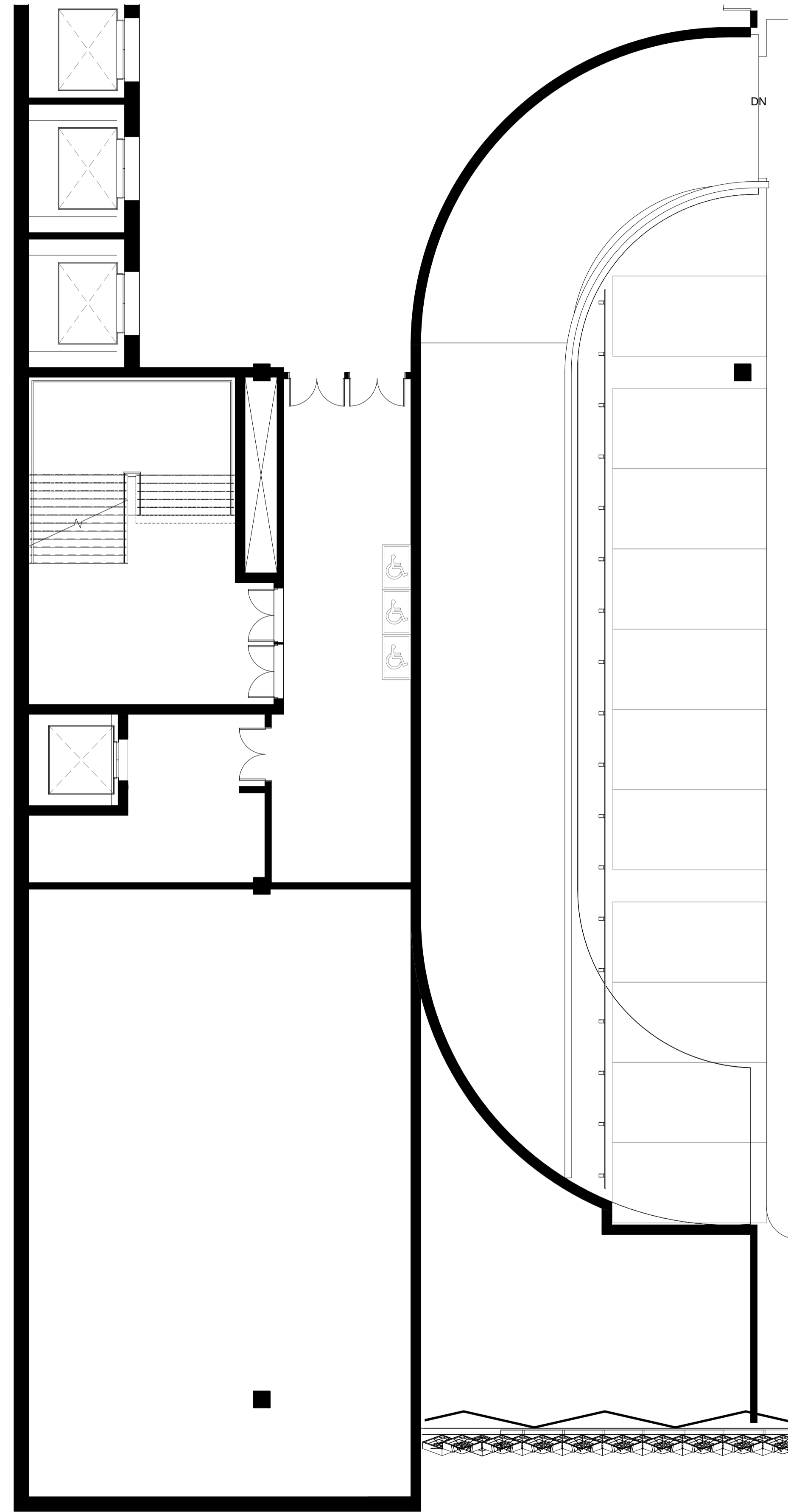
Community Study Plans - Level 5 (CP5) 1 : 100
