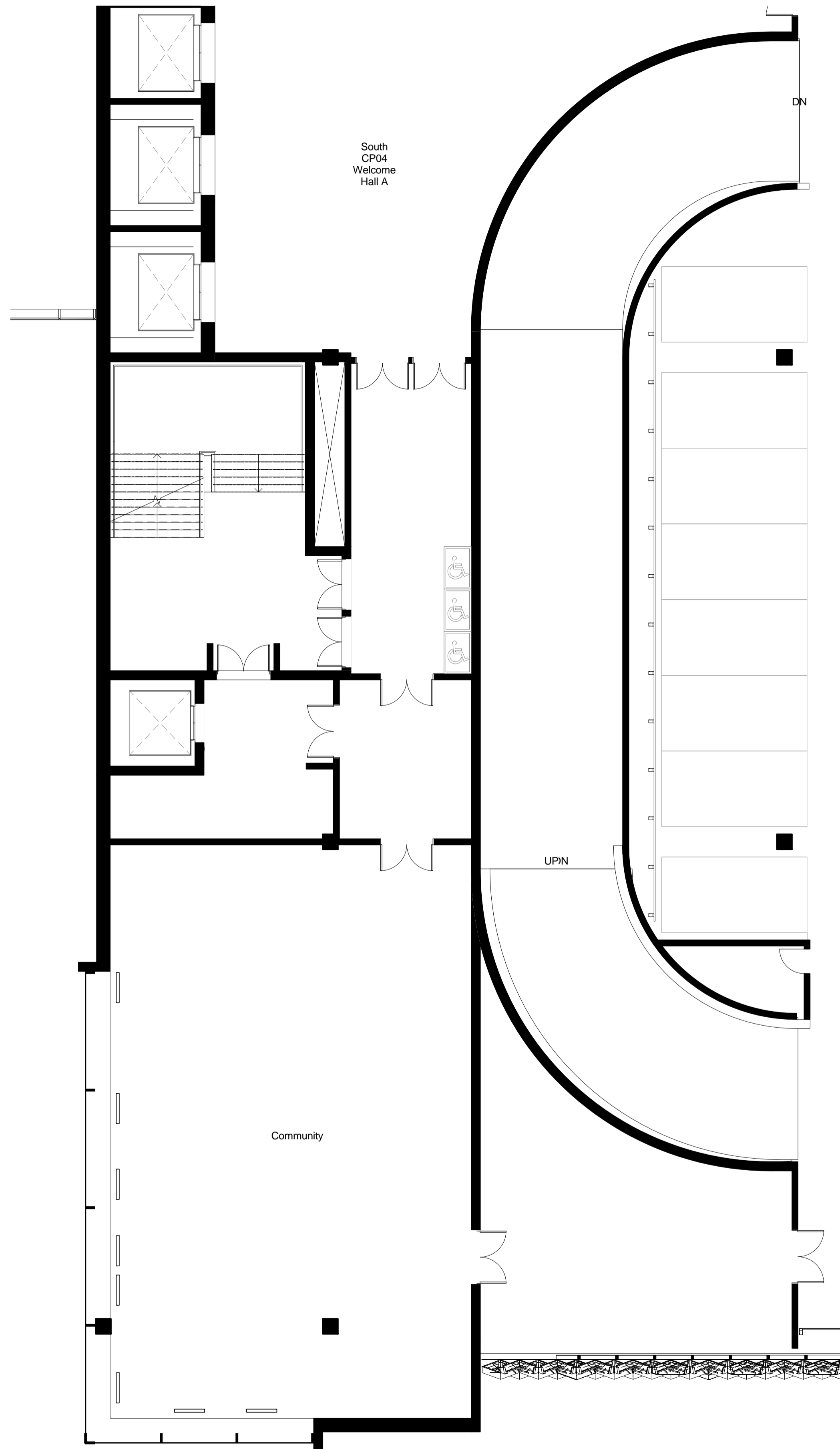
Community Study Plans - Level 4 (CP4) 1 : 100
