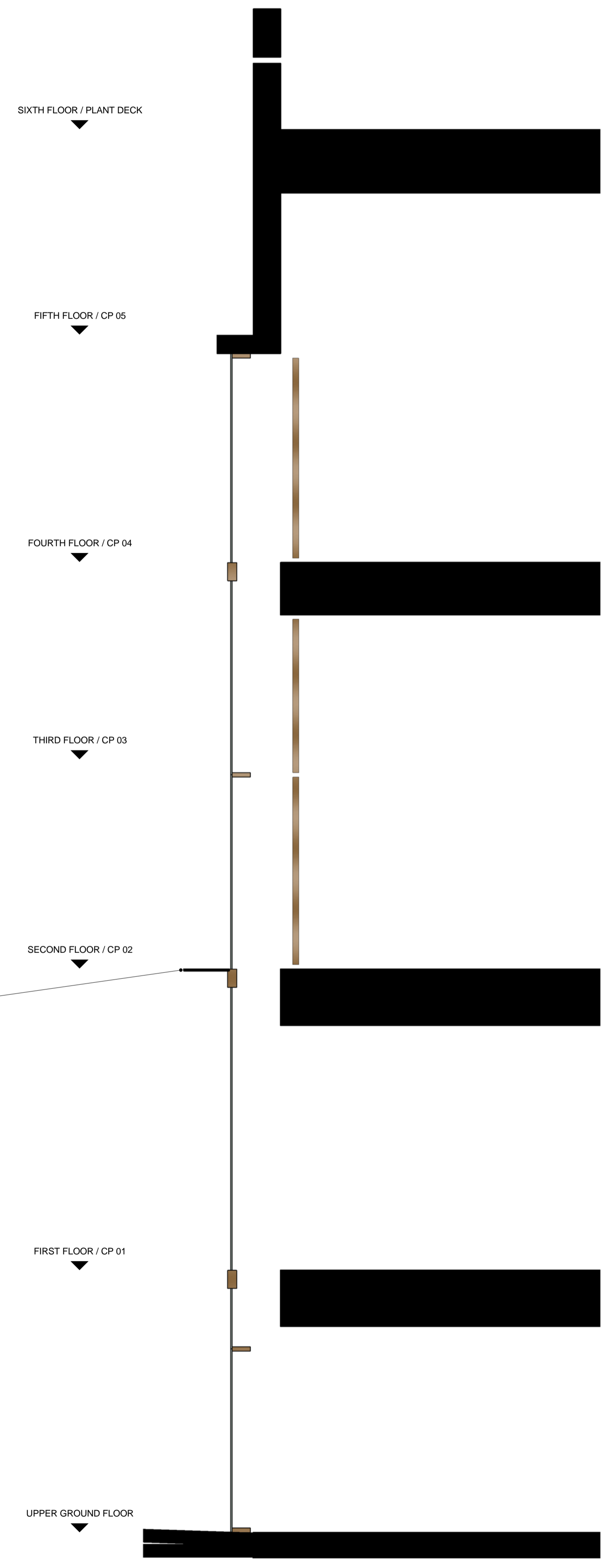
2 COMMUNITY FACADE SECTION 1 : 50
