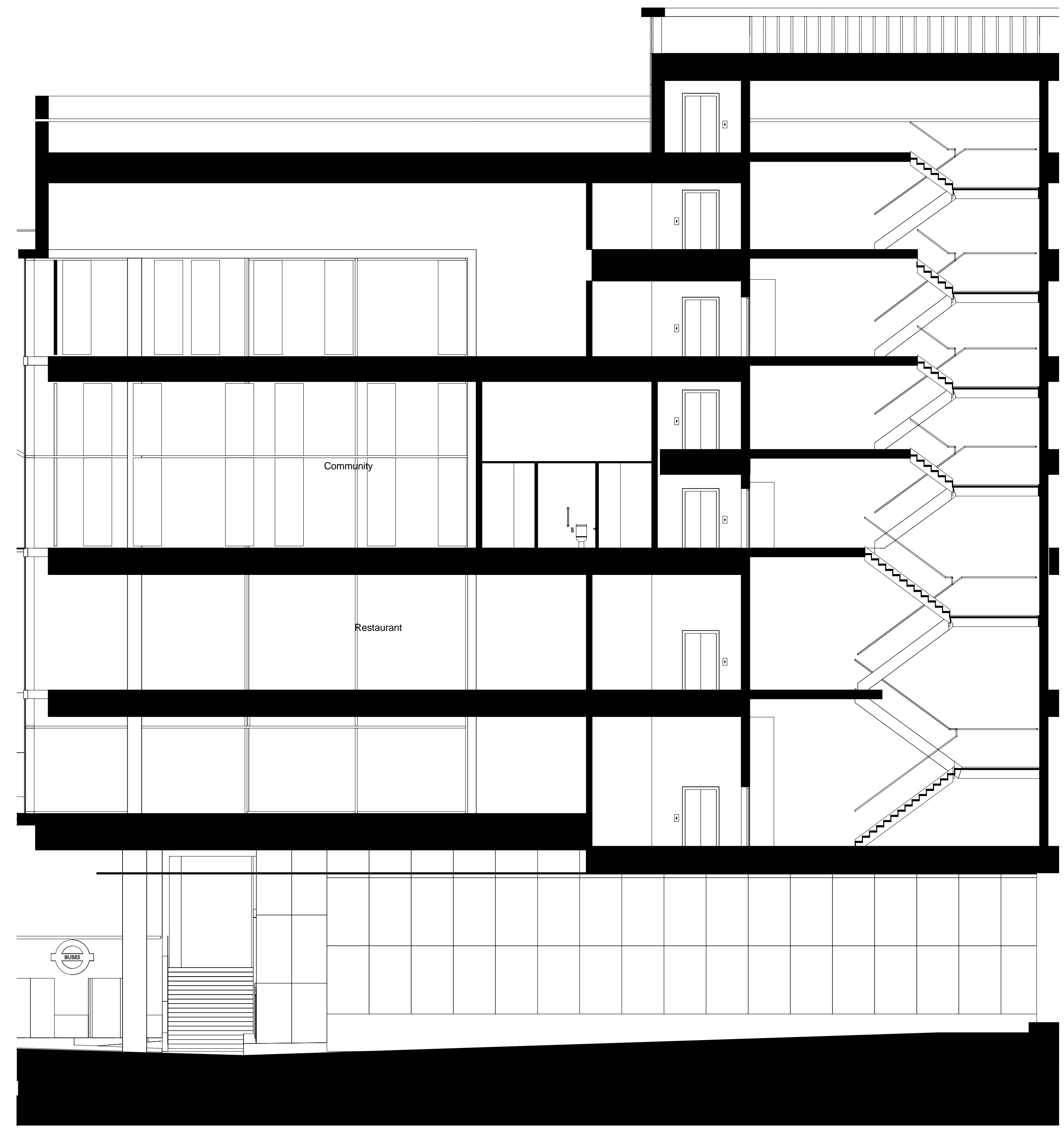
2 COMMUNITY STUDY SECTION 2 1 : 100
