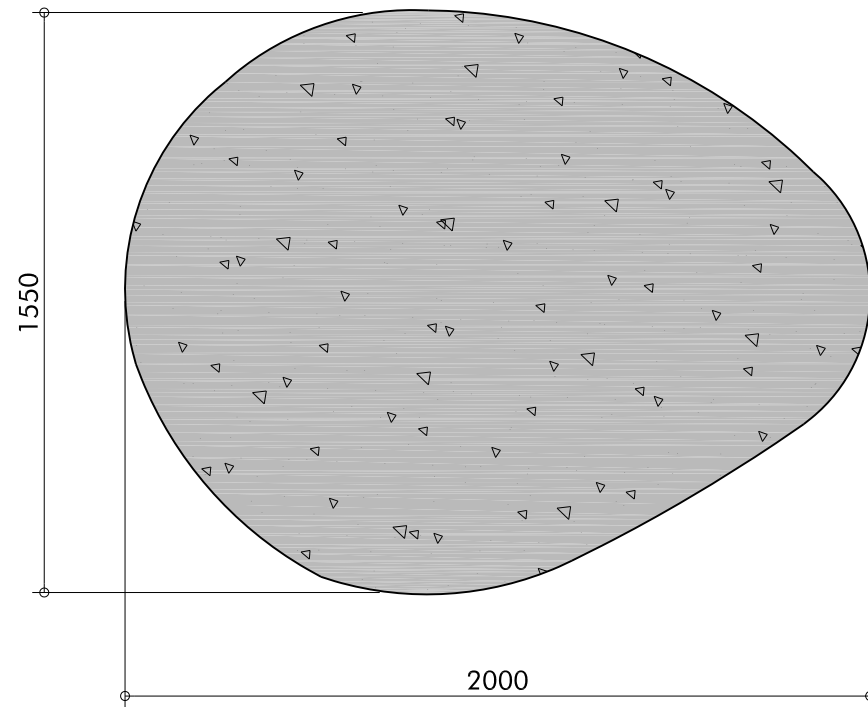
Plan 1:20@A3 Pebble Seat Type 1
