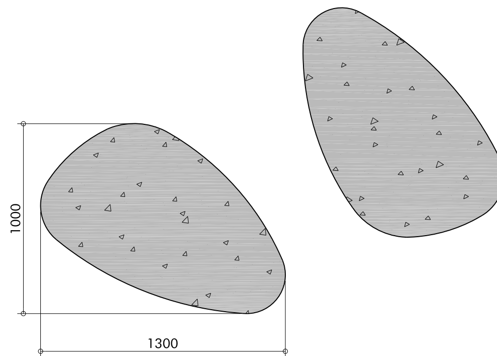
Plan 1:20@A3 Pebble Seat Type 2
