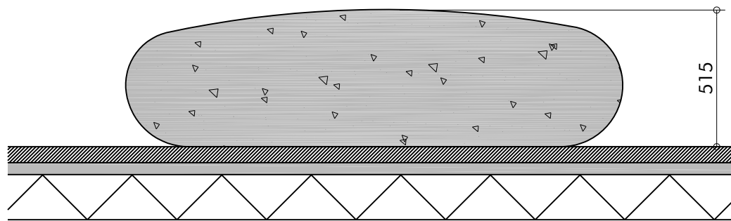
Elevation 1:20@A3 Pebble Seat Type 1
